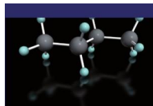
April 2014 Iminopropadienones The thermal generation and chemistry of iminopropadienone
