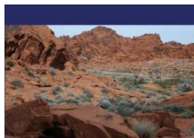
Piotr Nowinski Desert Varnish Indicator of Modern-Day Air Pollution
